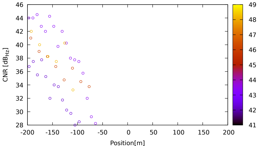
CNR vs position for R01 (G1) on LeicaGS15 - DOY 262 jam. 1
