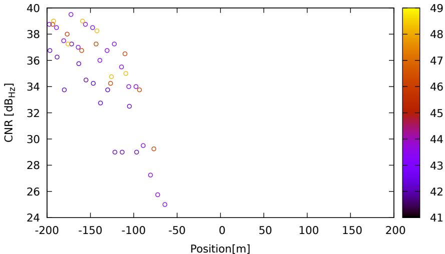
CNR vs position for R01 (G2) on LeicaGS15 - DOY 262 jam. 1
