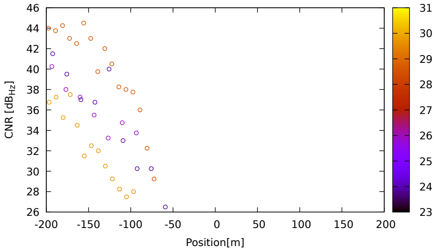
CNR vs position for R07 (G1) on LeicaGS15 - DOY 262 jam. 1
