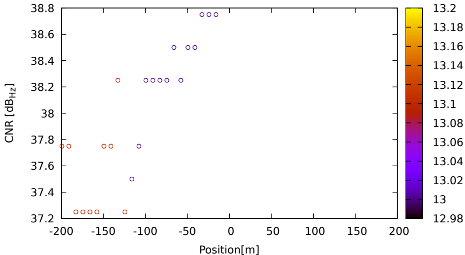
CNR vs position for R07 (G2) on LeicaGS15 - DOY 262 jam. 3
