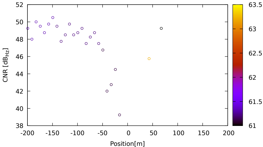
CNR vs position for R08 (G1) on LeicaGS15 - DOY 262 jam. 3
