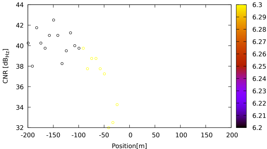
CNR vs position for R09 (G1) on LeicaGS15 - DOY 262 jam. 3
