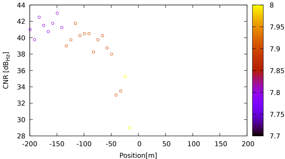
CNR vs position for R17 (G1) on LeicaGS15 - DOY 262 jam. 3
