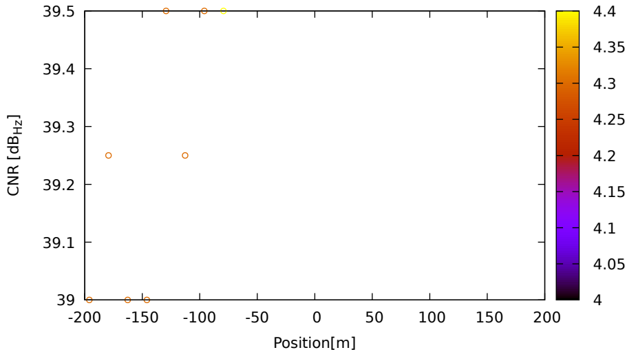
CNR vs position for R17 (G2) on LeicaGS15 - DOY 262 jam. 2
