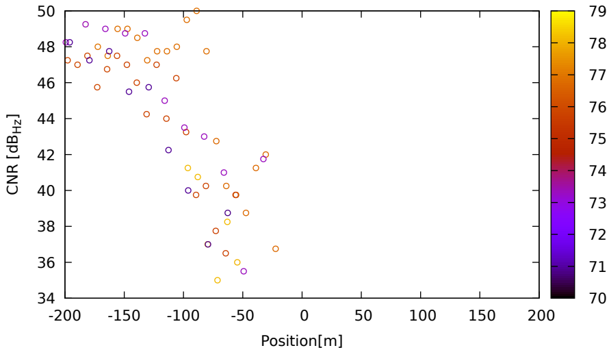
CNR vs position for R23 (G1) on LeicaGS15 - DOY 262 jam. 2
