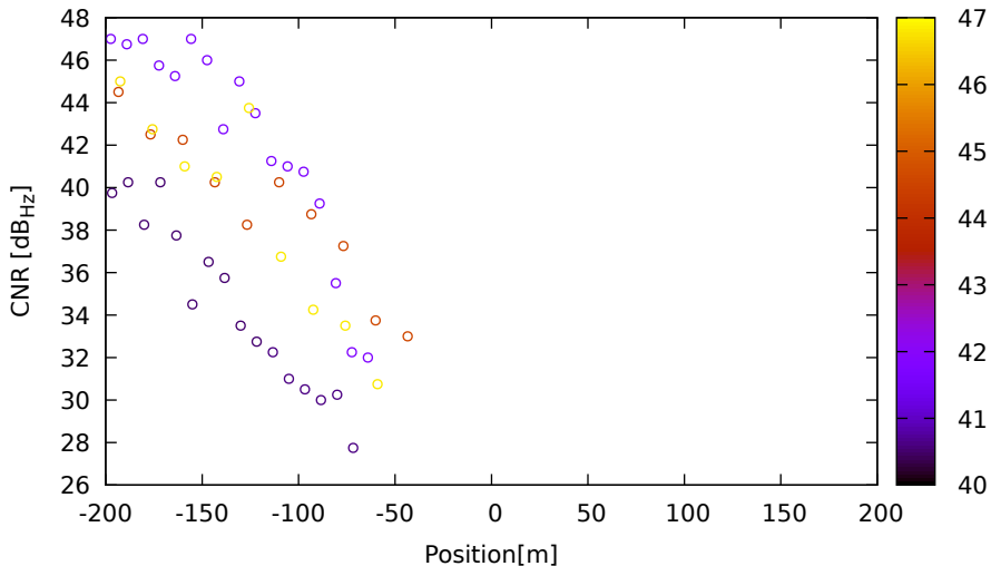
CNR vs position for R24 (G1) on LeicaGS15 - DOY 262 jam. 1
