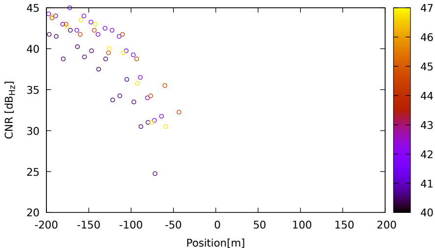
CNR vs position for R24 (G2) on LeicaGS15 - DOY 262 jam. 1
