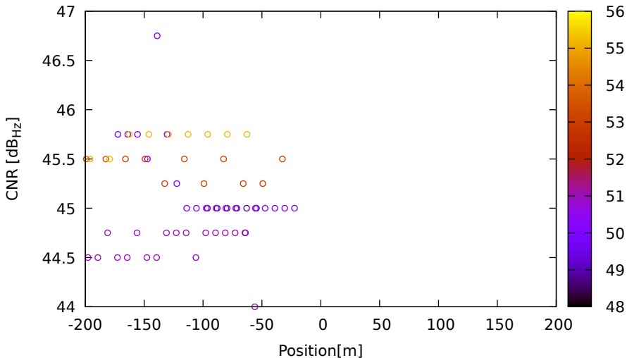
CNR vs position for R24 (G2) on LeicaGS15 - DOY 262 jam. 2
