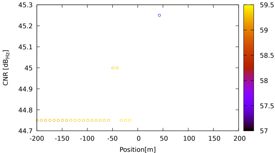
CNR vs position for R24 (G2) on LeicaGS15 - DOY 262 jam. 3
