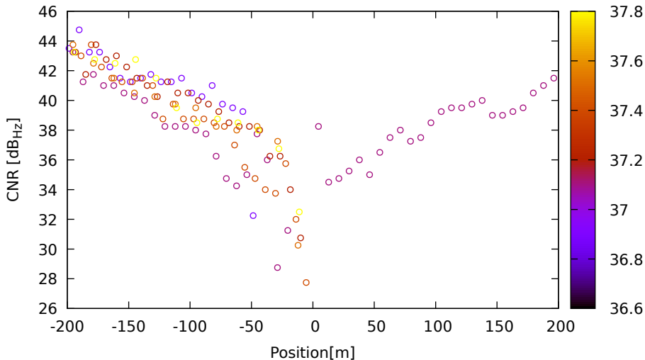
CNR vs position for C09 (B1) on LeicaGS18 - DOY 262 jam. 1
