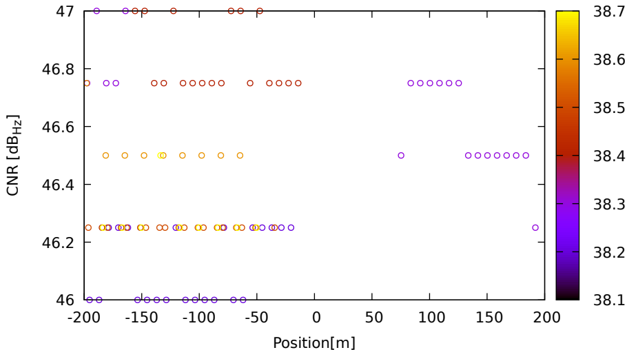
CNR vs position for C09 (B2) on LeicaGS18 - DOY 262 jam. 2
