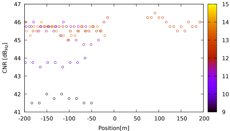
CNR vs position for C11 (B2) on LeicaGS18 - DOY 262 jam. 2
