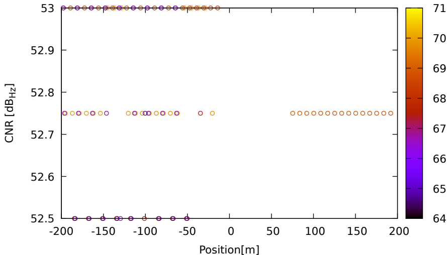
CNR vs position for C14 (B2) on LeicaGS18 - DOY 262 jam. 2
