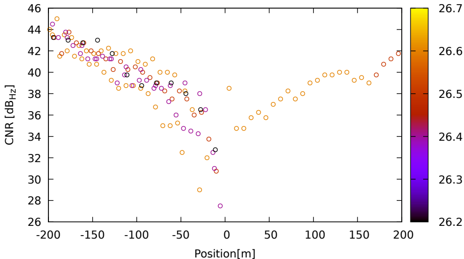
CNR vs position for C16 (B1) on LeicaGS18 - DOY 262 jam. 1
