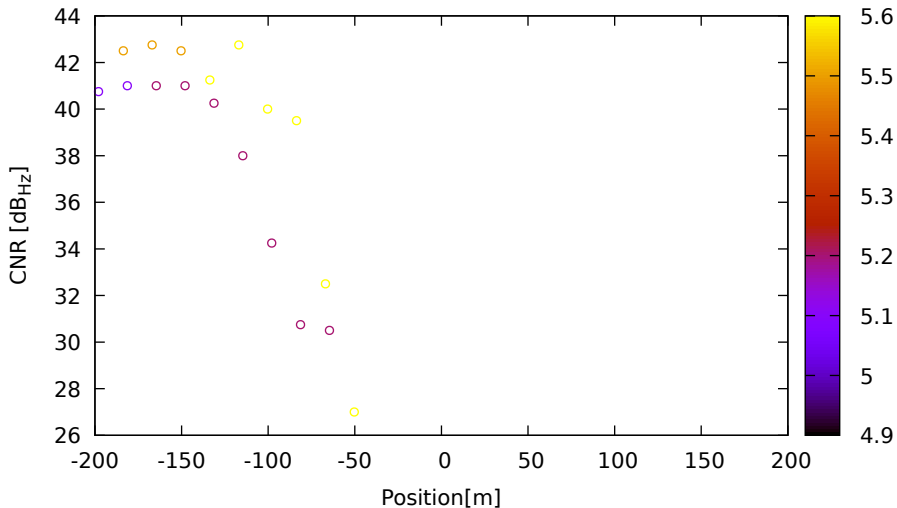
CNR vs position for C26 (B1) on LeicaGS18 - DOY 262 jam. 2
