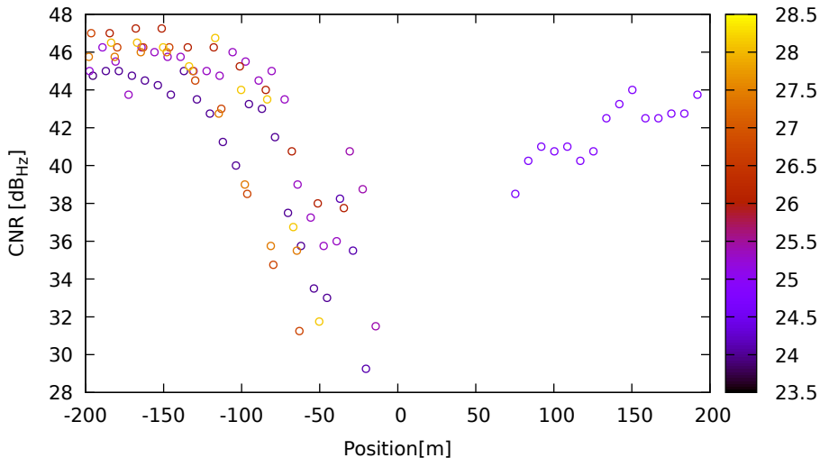
CNR vs position for C27 (B1) on LeicaGS18 - DOY 262 jam. 2
