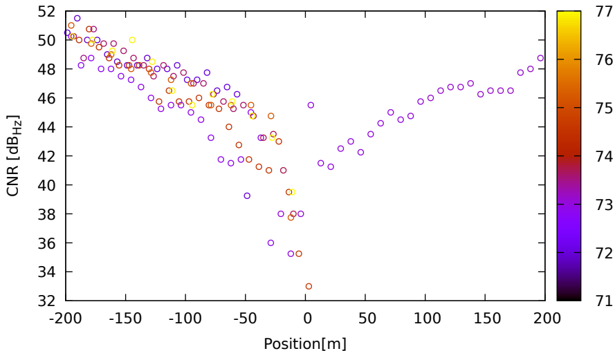
CNR vs position for C33 (B1) on LeicaGS18 - DOY 262 jam. 1
