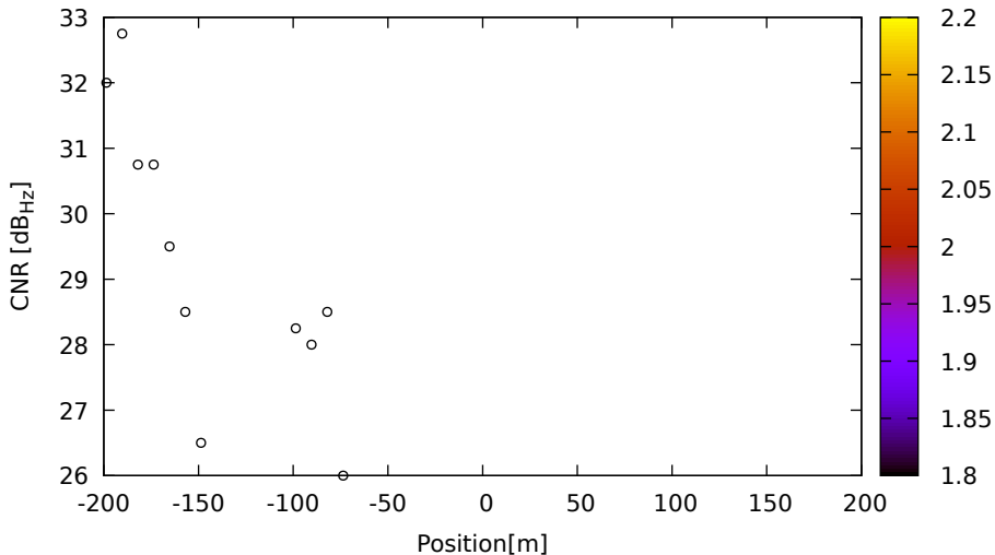
CNR vs position for C34 (B1) on LeicaGS18 - DOY 262 jam. 1
