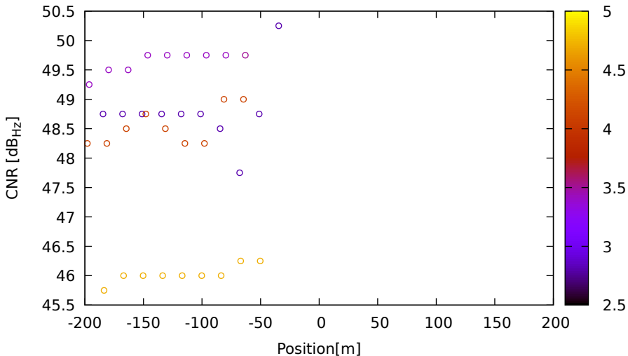
CNR vs position for E03 (E5) on LeicaGS18 - DOY 262 jam. 2
