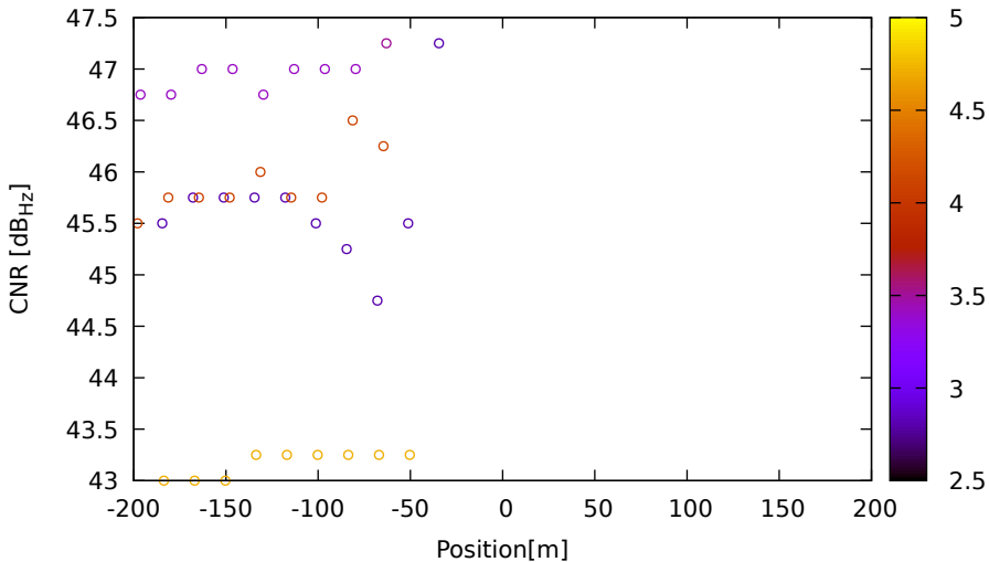
CNR vs position for E03 (E5b) on LeicaGS18 - DOY 262 jam. 2
