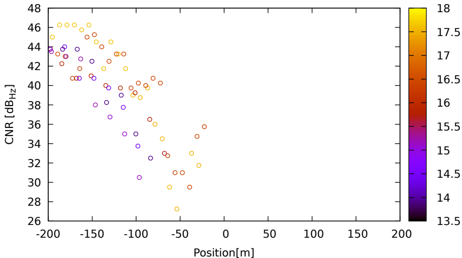
CNR vs position for E04 (E1) on LeicaGS18 - DOY 262 jam. 2
