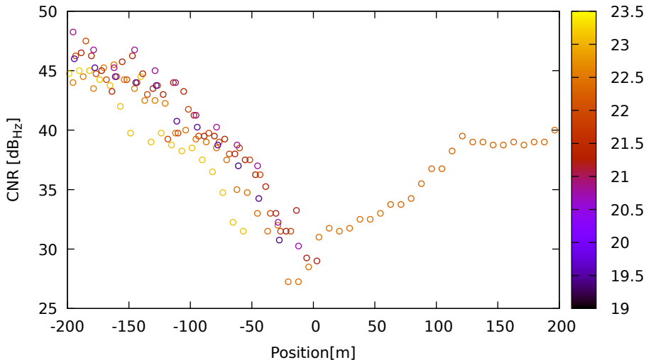
CNR vs position for E04 (E5) on LeicaGS18 - DOY 262 jam. 1
