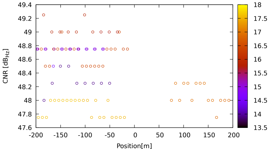
CNR vs position for E04 (E5) on LeicaGS18 - DOY 262 jam. 2
