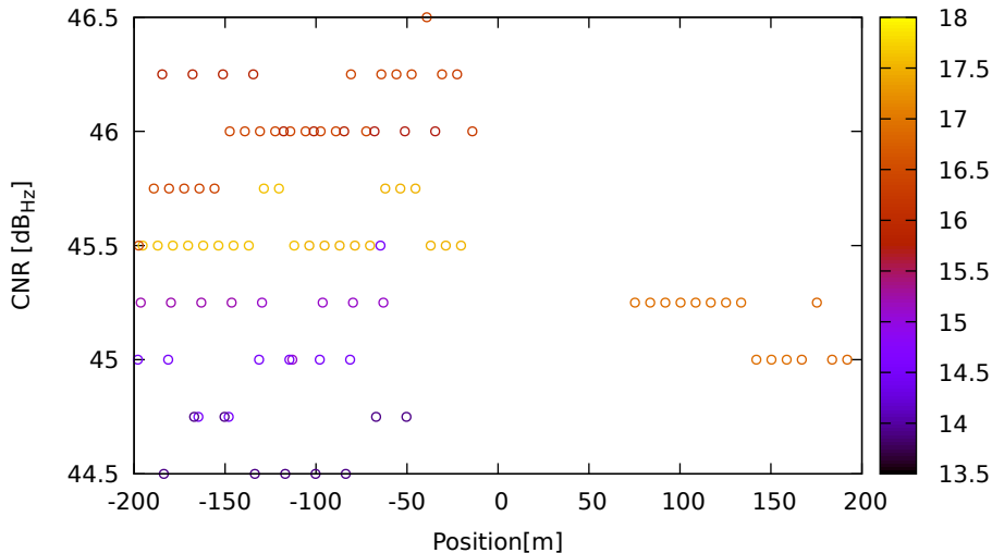
CNR vs position for E04 (E5a) on LeicaGS18 - DOY 262 jam. 2
