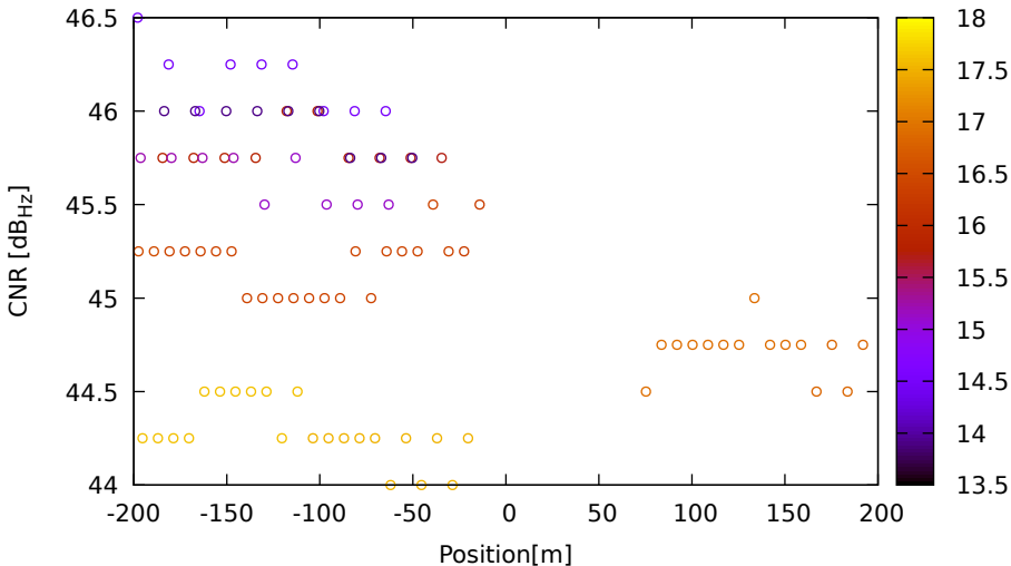
CNR vs position for E04 (E5b) on LeicaGS18 - DOY 262 jam. 2
