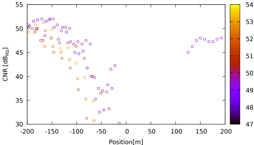
CNR vs position for E05 (E1) on LeicaGS18 - DOY 262 jam. 2
