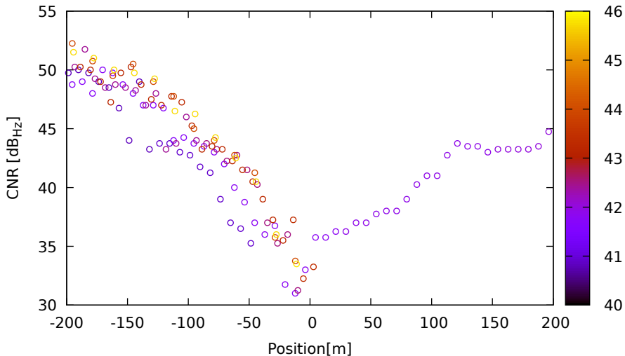
CNR vs position for E05 (E5) on LeicaGS18 - DOY 262 jam. 1
