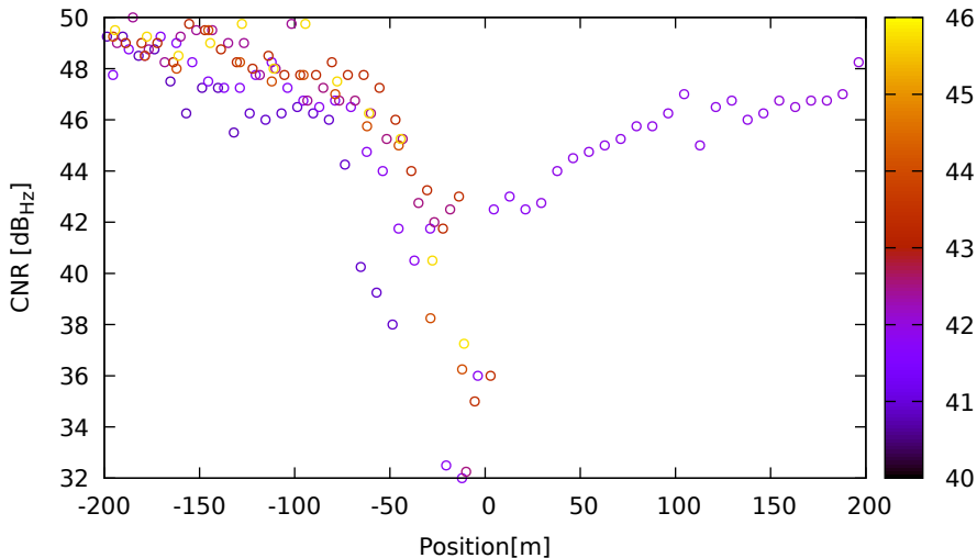
CNR vs position for E05 (E5a) on LeicaGS18 - DOY 262 jam. 1
