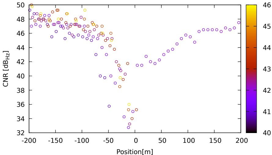
CNR vs position for E05 (E5b) on LeicaGS18 - DOY 262 jam. 1
