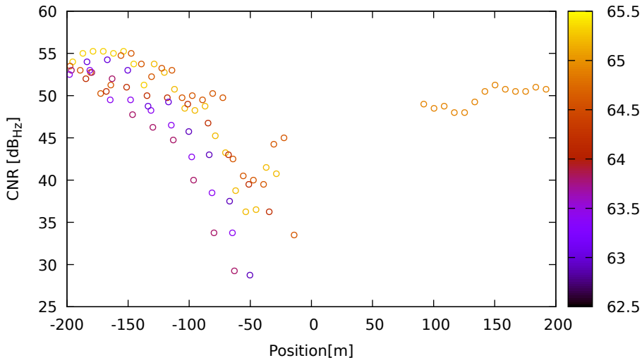
CNR vs position for E09 (E1) on LeicaGS18 - DOY 262 jam. 2
