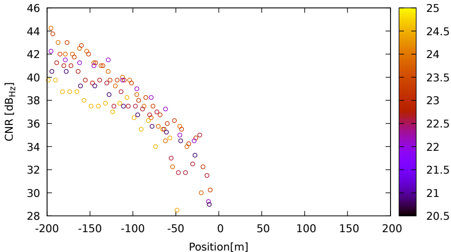
CNR vs position for E11 (E1) on LeicaGS18 - DOY 262 jam. 1
