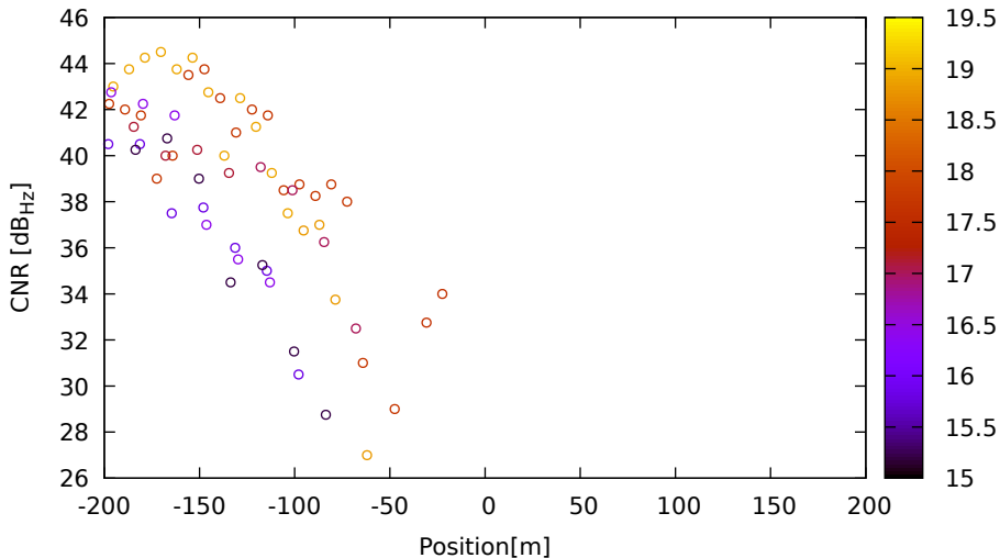
CNR vs position for E11 (E1) on LeicaGS18 - DOY 262 jam. 2
