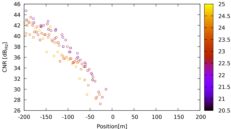
CNR vs position for E11 (E5) on LeicaGS18 - DOY 262 jam. 1
