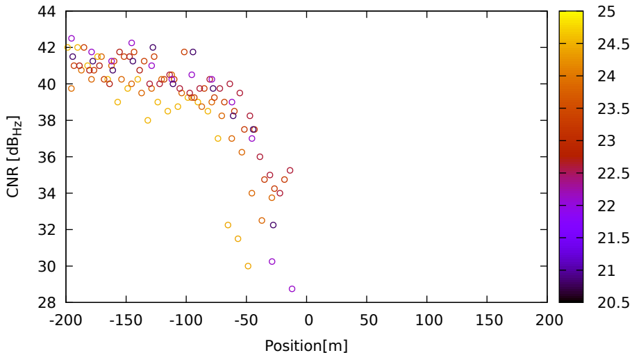
CNR vs position for E11 (E5a) on LeicaGS18 - DOY 262 jam. 1
