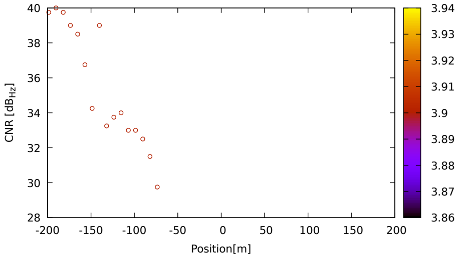
CNR vs position for E27 (E5) on LeicaGS18 - DOY 262 jam. 1
