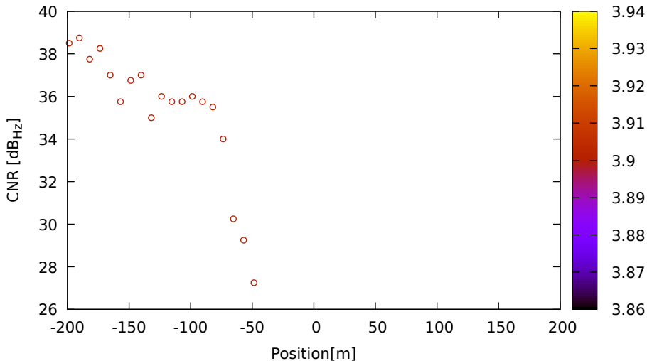
CNR vs position for E27 (E5a) on LeicaGS18 - DOY 262 jam. 1
