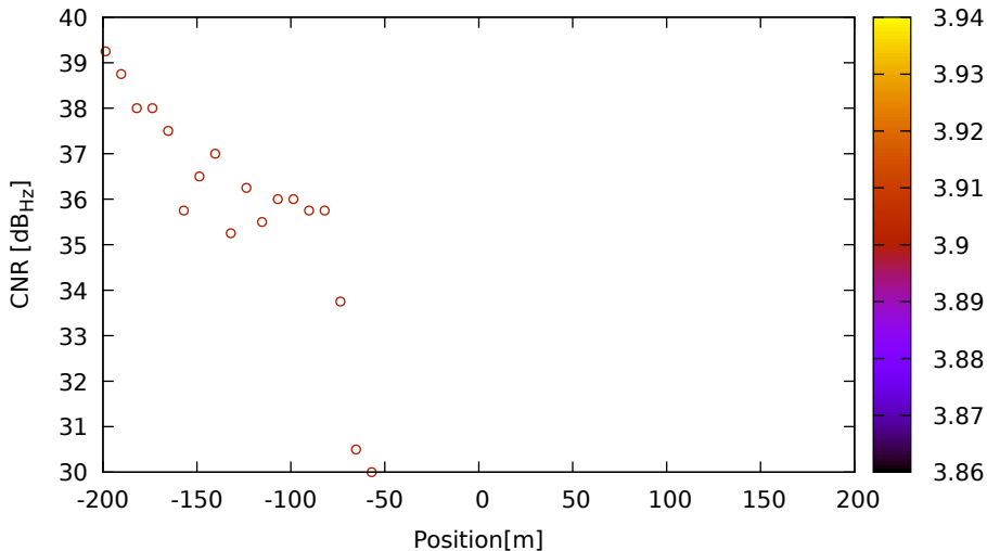
CNR vs position for E27 (E5b) on LeicaGS18 - DOY 262 jam. 1
