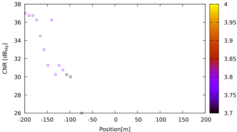
CNR vs position for E30 (E5) on LeicaGS18 - DOY 262 jam. 1
