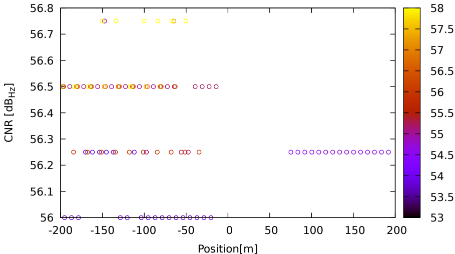
CNR vs position for E34 (E5) on LeicaGS18 - DOY 262 jam. 2
