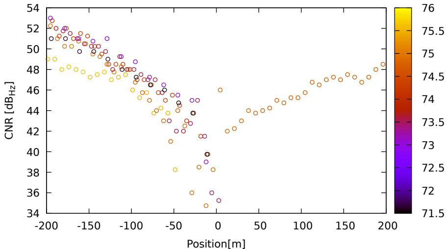
CNR vs position for E36 (E1) on LeicaGS18 - DOY 262 jam. 1
