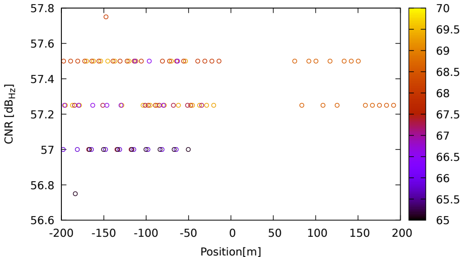
CNR vs position for E36 (E5) on LeicaGS18 - DOY 262 jam. 2
