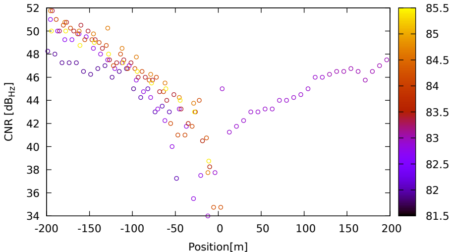
CNR vs position for G01 (L1) on LeicaGS18 - DOY 262 jam. 1
