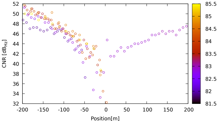
CNR vs position for G01 (L2) on LeicaGS18 - DOY 262 jam. 1
