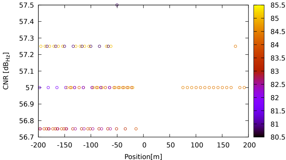
CNR vs position for G01 (L5) on LeicaGS18 - DOY 262 jam. 2
