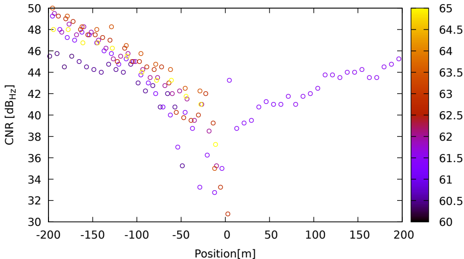
CNR vs position for G03 (L2) on LeicaGS18 - DOY 262 jam. 1
