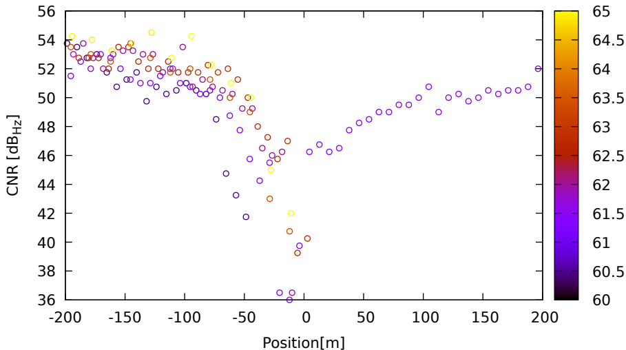
CNR vs position for G03 (L5) on LeicaGS18 - DOY 262 jam. 1
